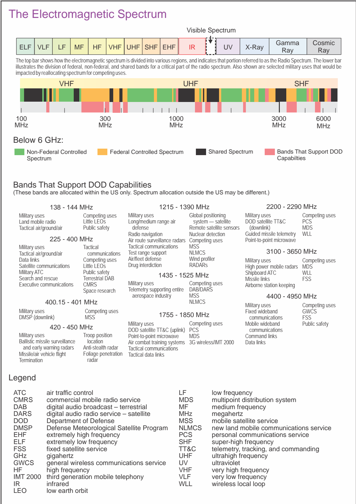
Figure I-2. The Electromagnetic Spectrum
