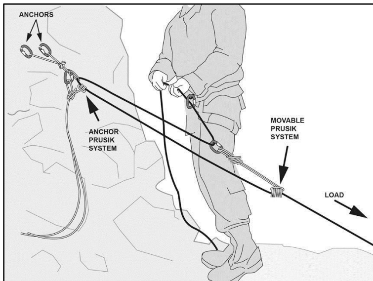
Figure 9-24. Z-Pulley system
