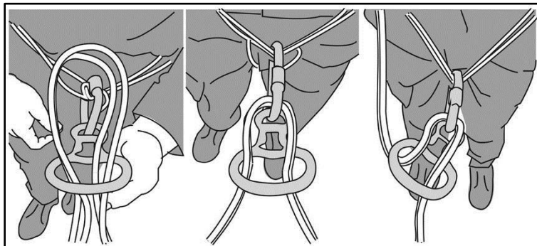
Figure 9-27. Figure-eight descender
