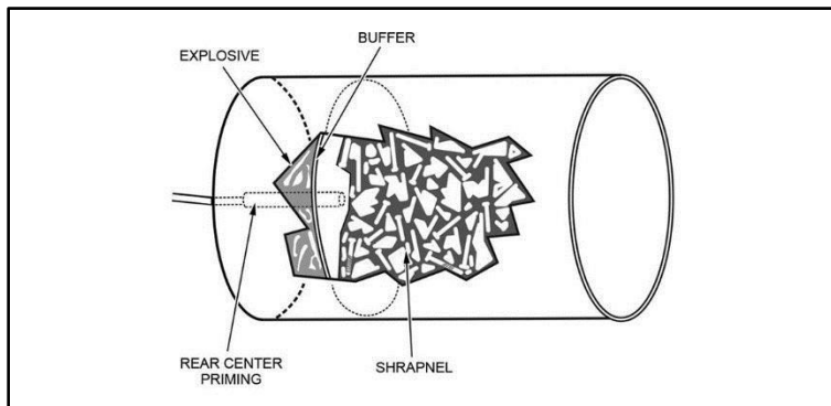
Figure 5-4. Grapeshot charge
