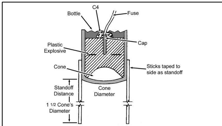
Figure 5-2. Improvised shape charge
