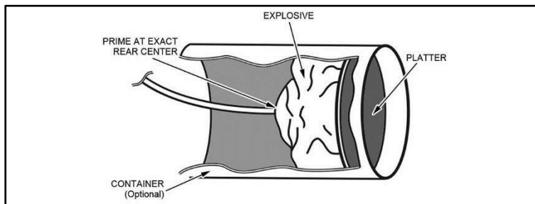
Figure 5-3. Platter charge
