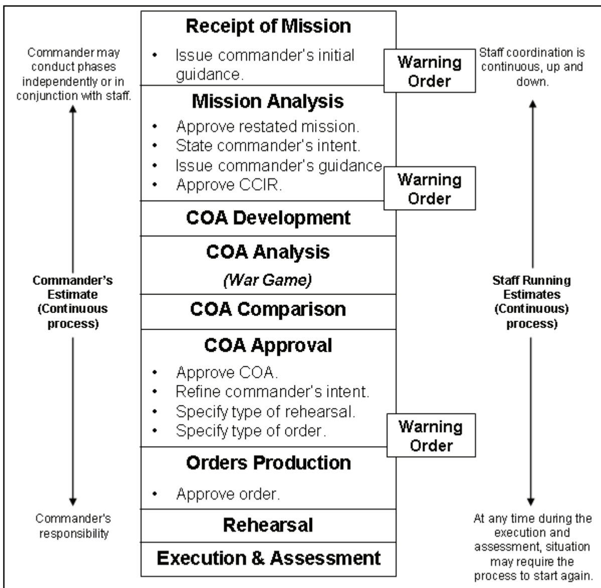
Figure 5-5. The MDMP
