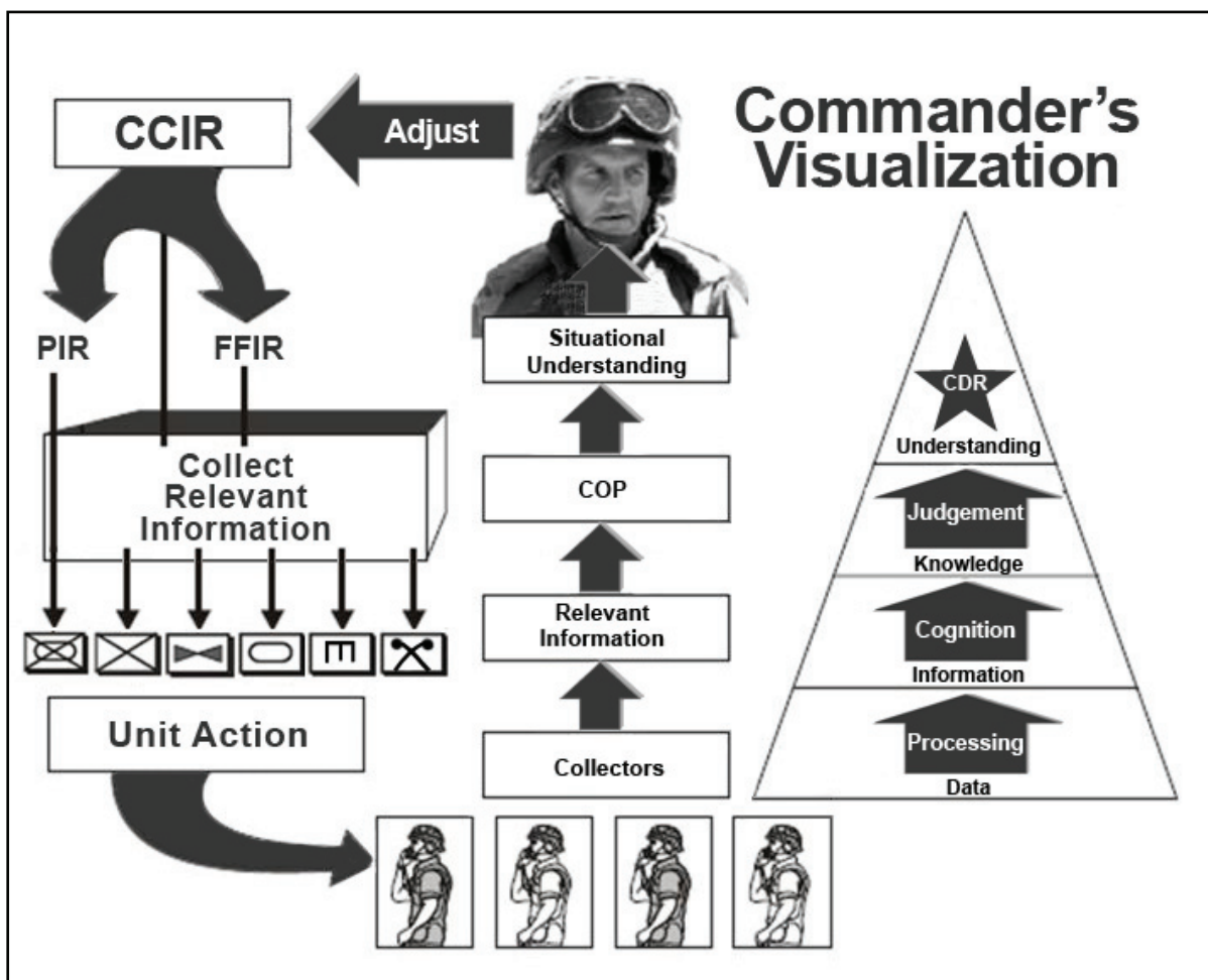
Figure 5-3. Developing SU
