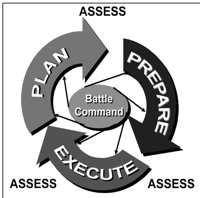
Figure 5-4. Operations process
