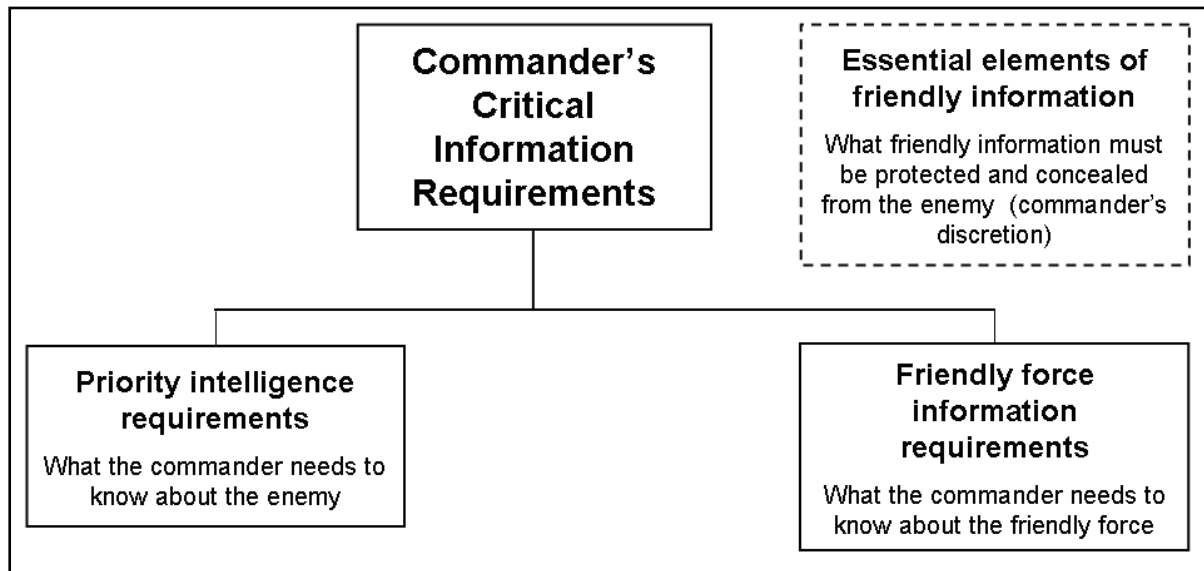
Figure 5-2. CCIR
