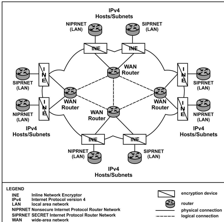
Figure 2-1. Colorless core architecture
