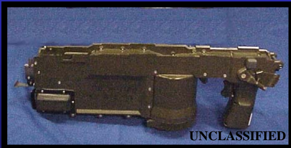
Gripstock
