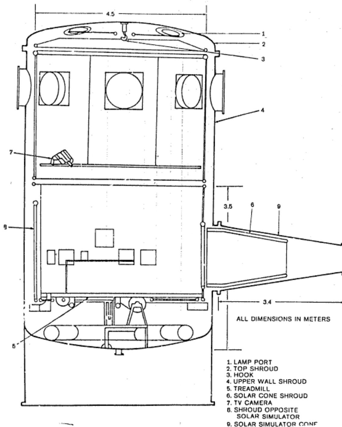
Figure 3. Cutaway Drawing of Vertical Chamber
