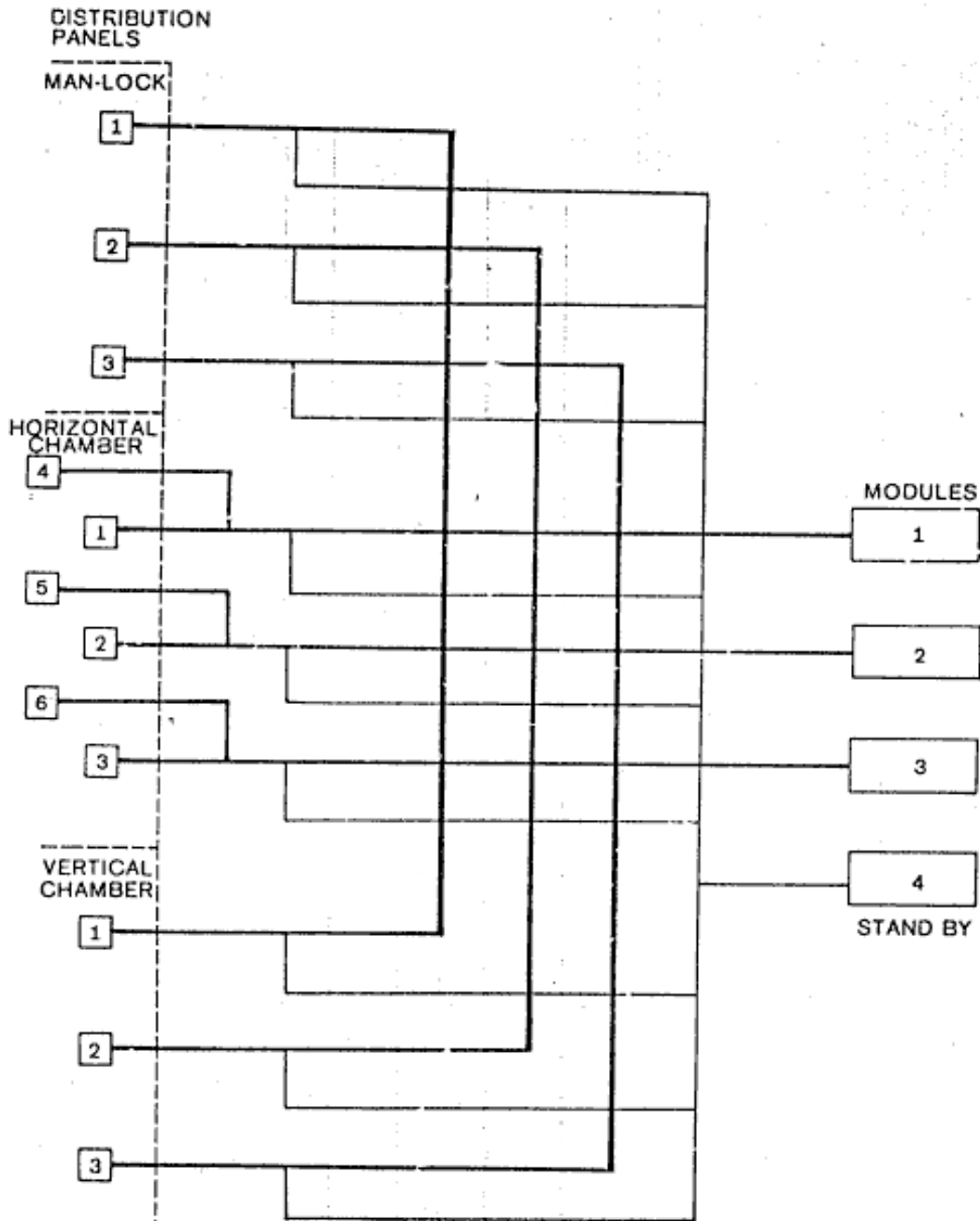
Figure 4. Oxygen System
