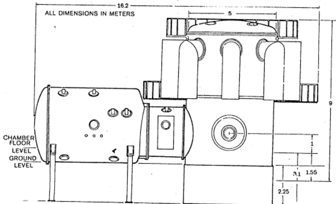
Figure 2. Schematic Drawing of Hypobaric Chamber
