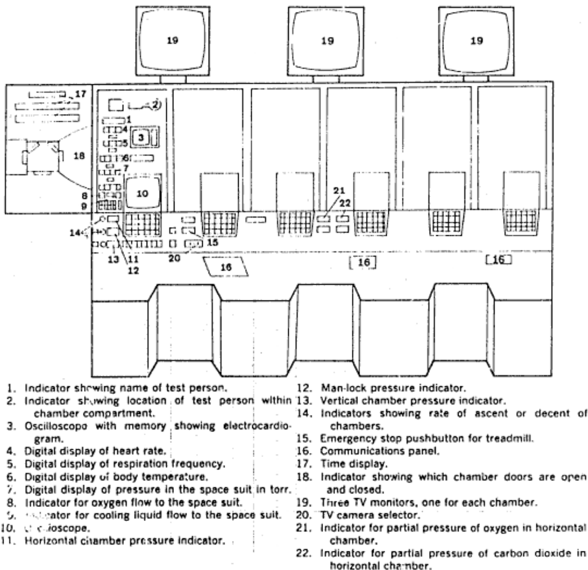
Figure 6. Doctor Operator Panel
