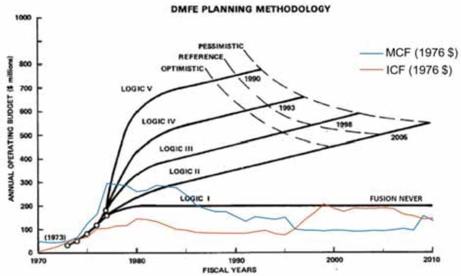
Figure 15. 1976 ERDA projections of routes to MCF fusion energy and historical fusion funding in 1976 dollars.
