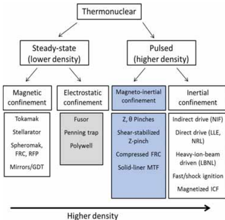
Figure 4. Approaches to controlled fusion. Thermonuclear approaches maintain an approximately Maxwell-Boltzmann velocity distribution, permitting each ion to undergo many Coulomb scattering events prior to a fusion reaction. MIF approaches are shaded in blue. Approaches unlikely to reach scientific break-even are shaded in grey. Image adapted from S. Hsu, LANL.
