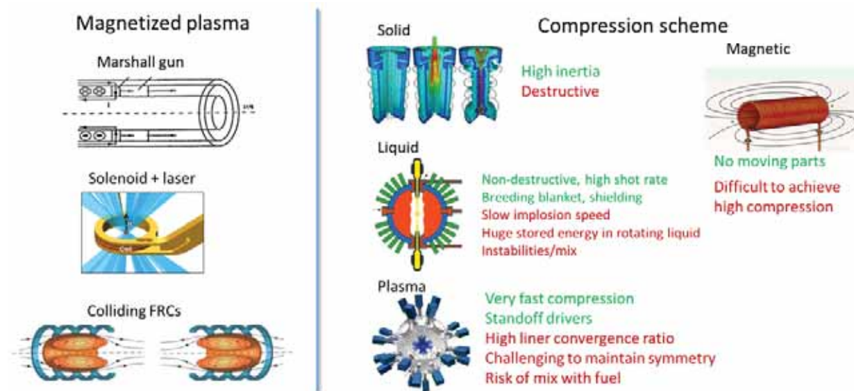
Figure 9. Ingredients of a MIF system. Many combinations of magnetized plasma and compression scheme are possible (though not all possibilities are practical). Only a subset of the plausible approaches has been tried.
