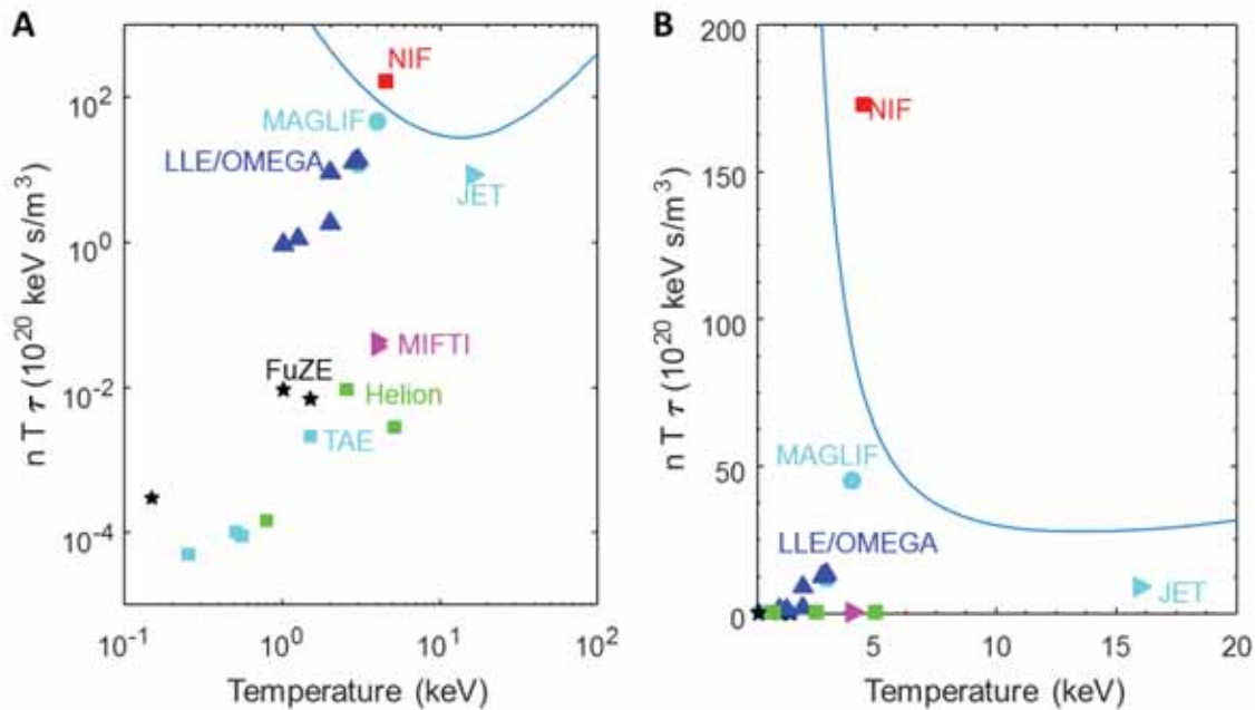
Figure 10. MIF efforts toward scientific break-even (blue curve). Tokamak programs (JET) and the NIF are included for comparison. A) Experimental results plotted on a log-log scale, as is customary. B) Same data plotted on a linear scale, highlighting the distance between most MIF programs and scientific break-even conditions.
