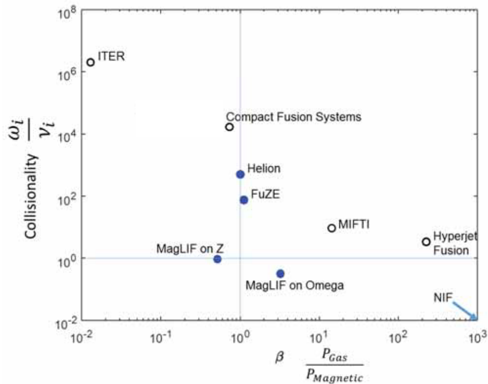
Figure 12. Fusion efforts arranged by dimensionless parameters. Empty circles represent projections, filled circles represent data. Parameters are approximate and are drawn from literature sources and communications with the project leads.
