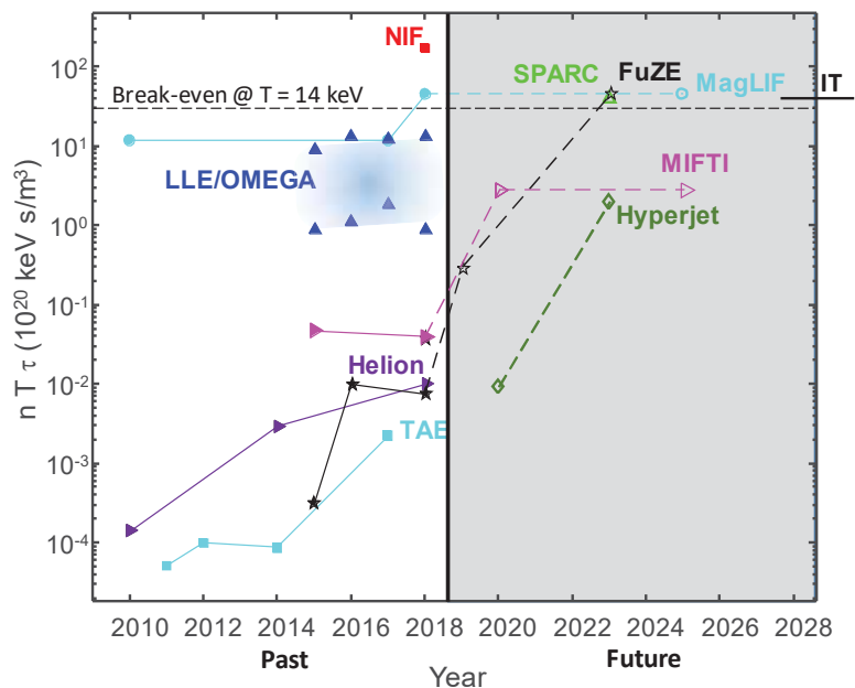
Figure 11. MIF progress vs. time toward scientific break-even. Filled symbols represent past results, empty symbols represent future projections. Tokamak programs (ITER, SPARC) and the NIF are included for comparison. The indicated break-even condition is specific to T = 14 keV. MagLIF did not achieve break-even despite crossing this threshold in triple product because MagLIF was too cold.
