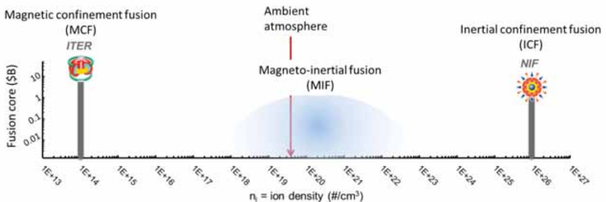
Figure 1. Fusion landscape. Magneto-inertial fusion resides at an intermediate density between Magnetic Confinement Fusion (MCF) and Inertial Confinement Fusion (ICF). Image adapted from P. McGrath, ARPA-E.
