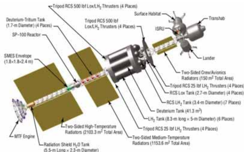
Figure 13. HOPE spacecraft design.
