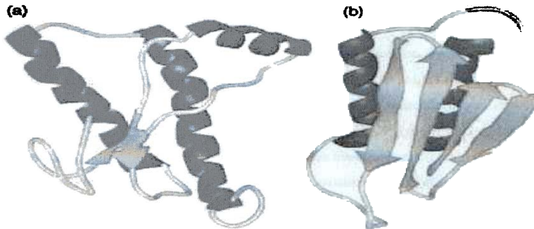
Figure 2. Ribbon diagrams depicting the secondary structure of PrP-sen (a) and PrP-sc (b); adapted from Cohen, F., 1999, Protein Misfolding and Prion Diseases, The Journal of Molecular Biology, 293, pp. 313-320. Arrows depict \beta -strands and helices depict \alpha -helices.
