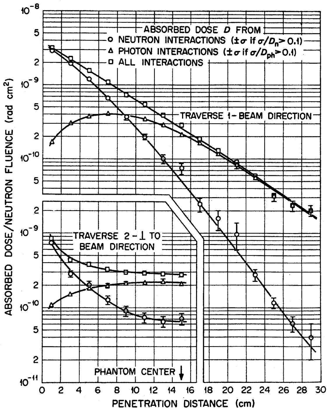
Figure 2. Absorbed dose per neutron fluence vs. depth in central region of 30-cm diameter cylindrical phantom of tissue-equivalent material at incident neutron energy of 1 MeV (NCRP, 1971; Figure 15).
