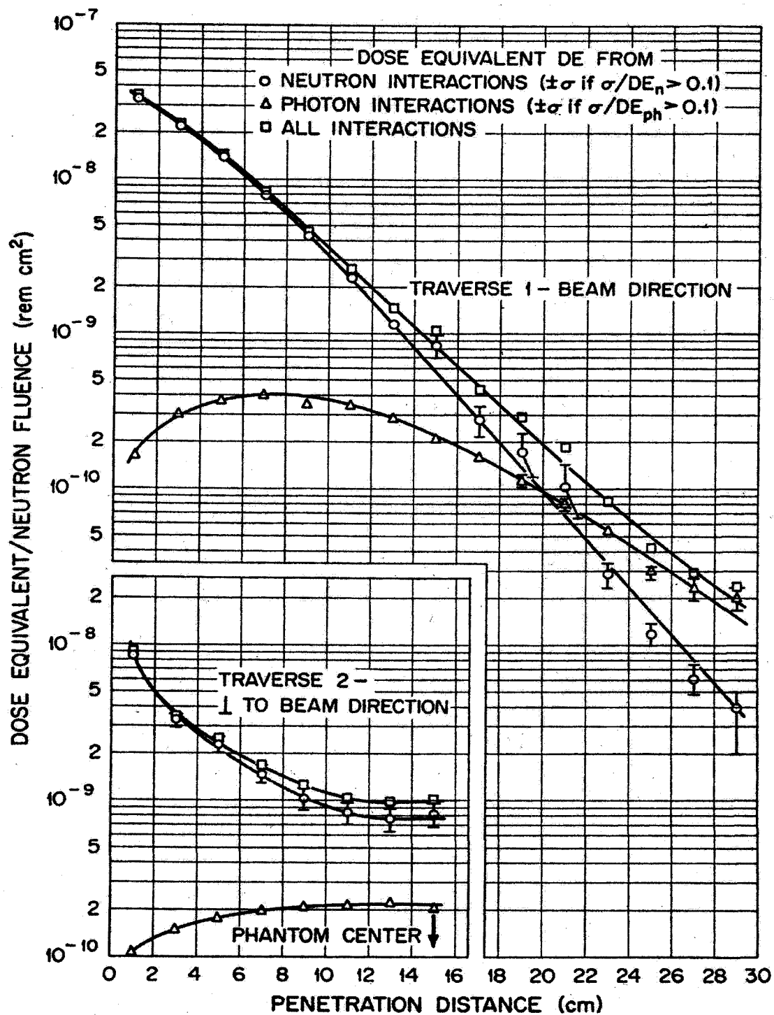
Figure 3. Dose equivalent per neutron fluence vs. depth in central region of 30-cm diameter cylindrical phantom of tissue-equivalent material at incident neutron energy of 1 MeV (NCRP, 1971; Figure 16).
