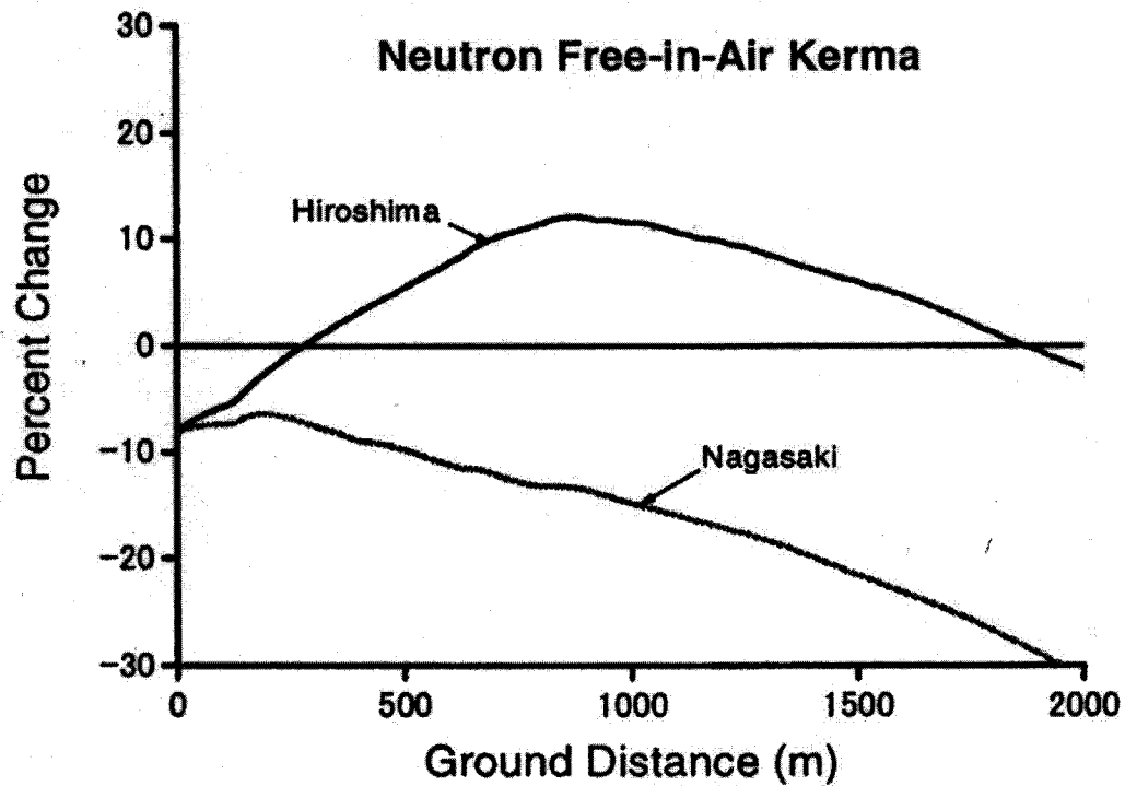
Figure 6. Changes in estimates of neutron kerma free-in-air vs. ground distance from detonations at Hiroshima and Nagasaki due to change in dosimetry system from DS86 to DS02 (Cullings and Fujita, 2003).
