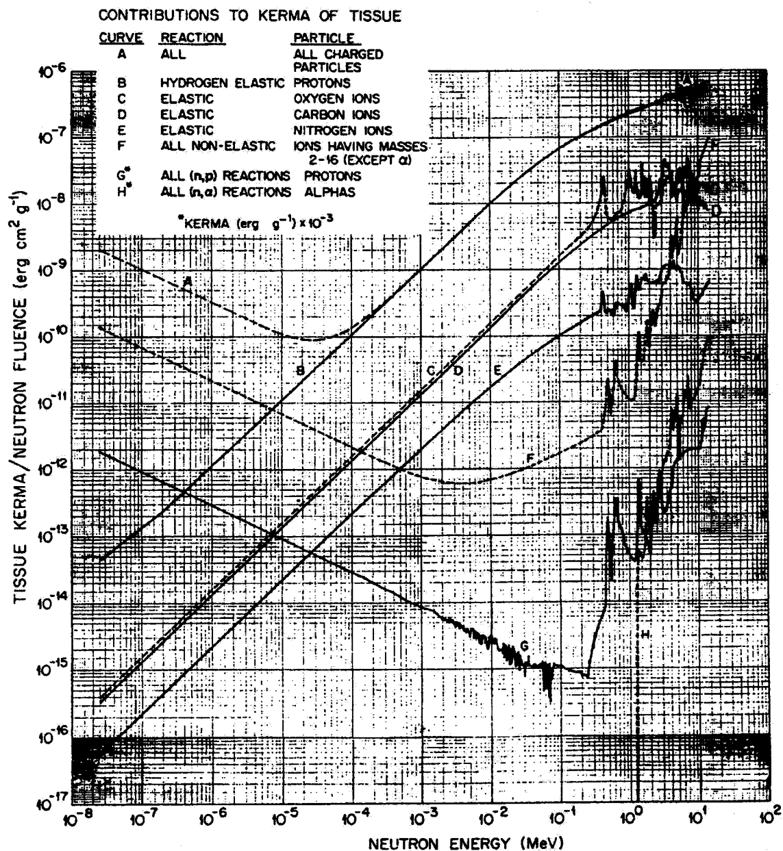
Figure 1. Tissue kerma free-in-air per neutron fluence and contributions from different reactions of neutrons with constituents of tissue vs. neutron energy (NCRP, 1971; Figure 3). To obtain kerma per neutron fluence in units of rad cm 2 , divide values in units of erg cm 2 g -1 by 100.
