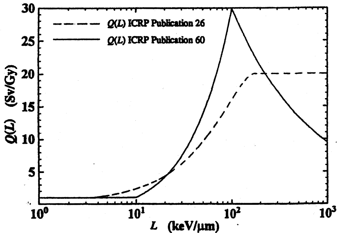
Figure 4. Quality factor ( Q ) for charged ionizing particles vs. linear energy transfer ( L ) recommended in ICRP Publication 60 (ICRP, 1991) and recommended previously in ICRP Publication 26 (ICRP, 1977); see also ICRP (1996; 2003).
