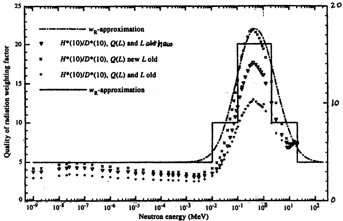
Figure 5. Summary of influence of relationship between quality factor ( Q ) and linear energy transfer ( L ) and stopping powers of charged particles on quality factor for neutrons (ICRP, 1996; Figure 3); new and old Q - L relationships are given in Figure 2-4. Data points are ratios of ambient dose equivalent and absorbed dose at depth of 1 cm in tissue, and solid and broken curves are recommendations on radiation weighting factors ( w_{RS} ) for neutrons given in Table 3-1 (ICRP, 1991). Scale on left vertical axis applies to all data points and curves, except scale on right vertical axis applies to data points obtained using old Q - L relationship and stopping-power data.
